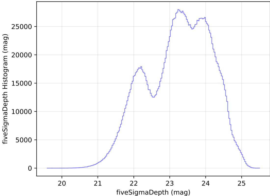
too_elab_r32_d3_ugrizy_v3.4_10yrs WFD all bands: fiveSigmaDepth Histogram
