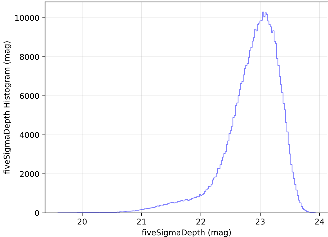
too_elab_r32_d3_ugrizy_v3.4_10yrs All sky z band: fiveSigmaDepth Histogram
