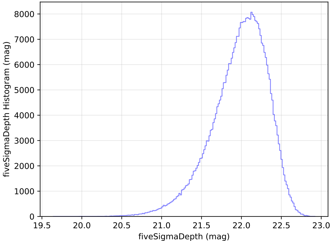
too_elab_r32_d3_ugrizy_v3.4_10yrs All sky y band: fiveSigmaDepth Histogram
