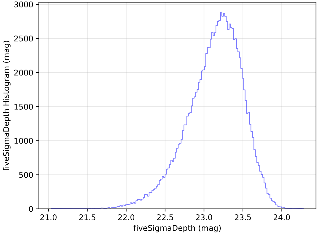
too_elab_r32_d3_ugrizy_v3.4_10yrs All sky u band: fiveSigmaDepth Histogram
