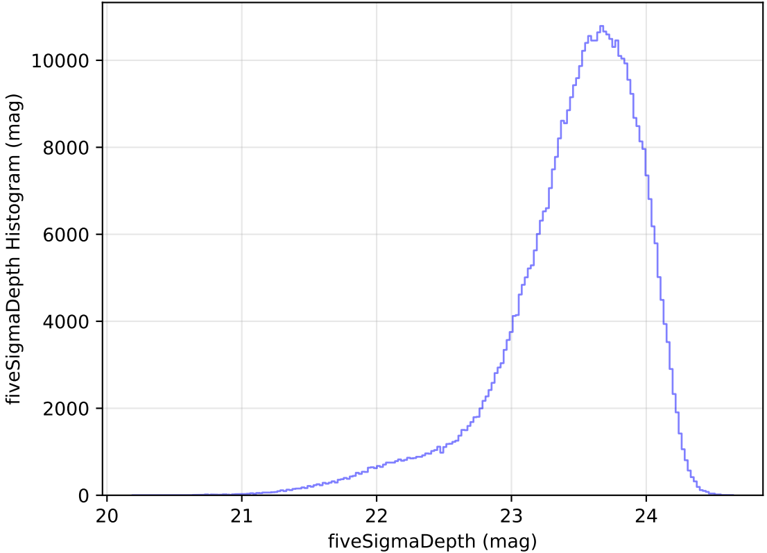
too_elab_r32_d3_ugrizy_v3.4_10yrs All sky i band: fiveSigmaDepth Histogram
