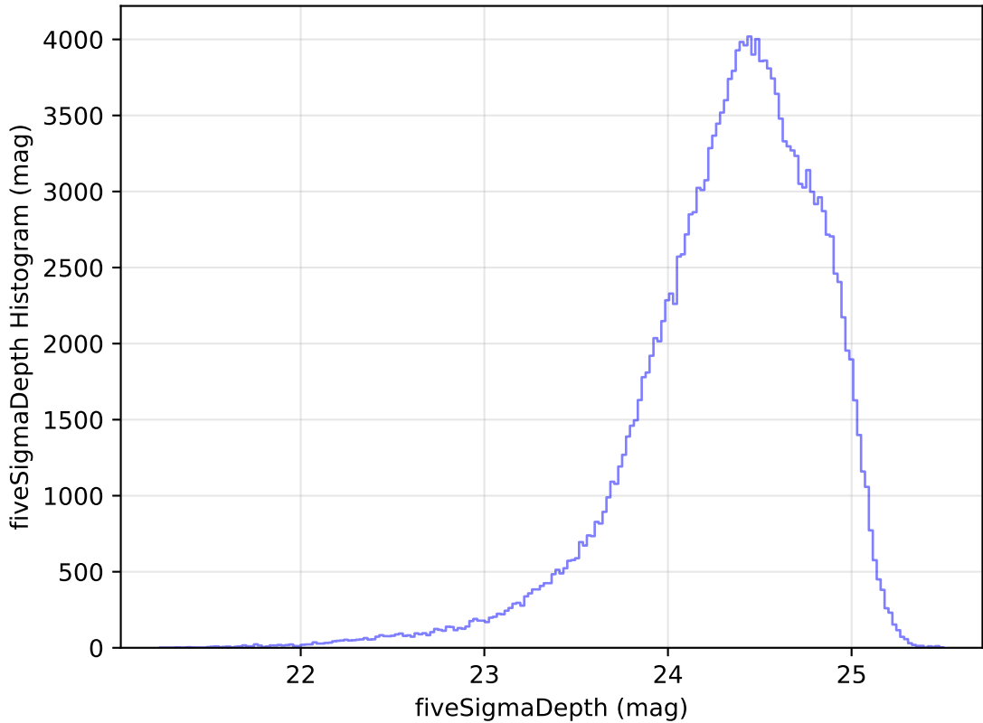
too_elab_r32_d3_ugrizy_v3.4_10yrs All sky g band: fiveSigmaDepth Histogram
