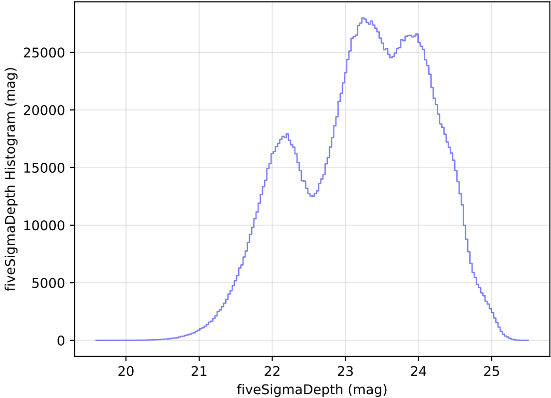
too_elab_r32_d3_ugrizy_v3.4_10yrs All sky all bands: fiveSigmaDepth Histogram
