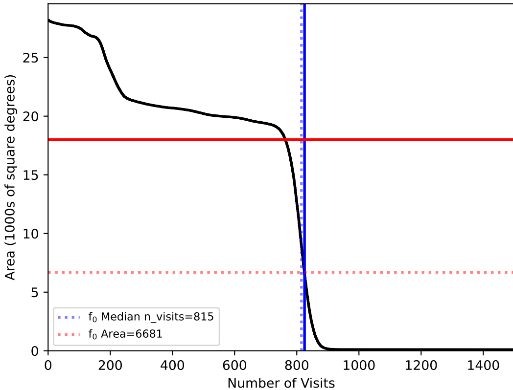
too_elab_r32_d3_ugrizy_v3.4_10yrs All sky: f0
