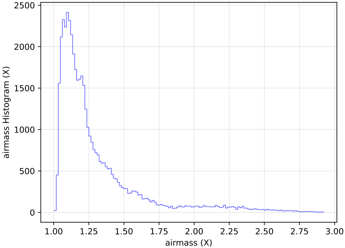
too_elab_r32_d3_ugrizy_v3.4_10yrs Yr 1 z band: airmass Histogram
