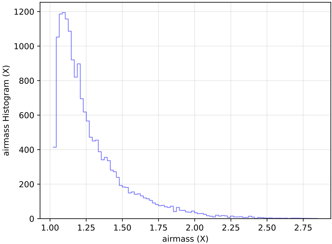
too_elab_r32_d3_ugrizy_v3.4_10yrs Yr 1 u band: airmass Histogram
