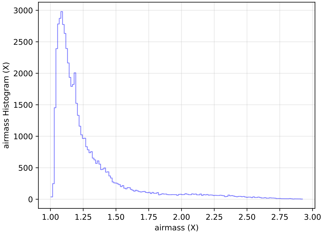
too_elab_r32_d3_ugrizy_v3.4_10yrs Yr 1 i band: airmass Histogram
