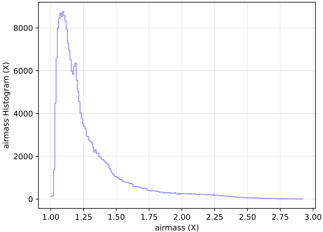
too_elab_r32_d3_ugrizy_v3.4_10yrs Yr 1 all bands: airmass Histogram
