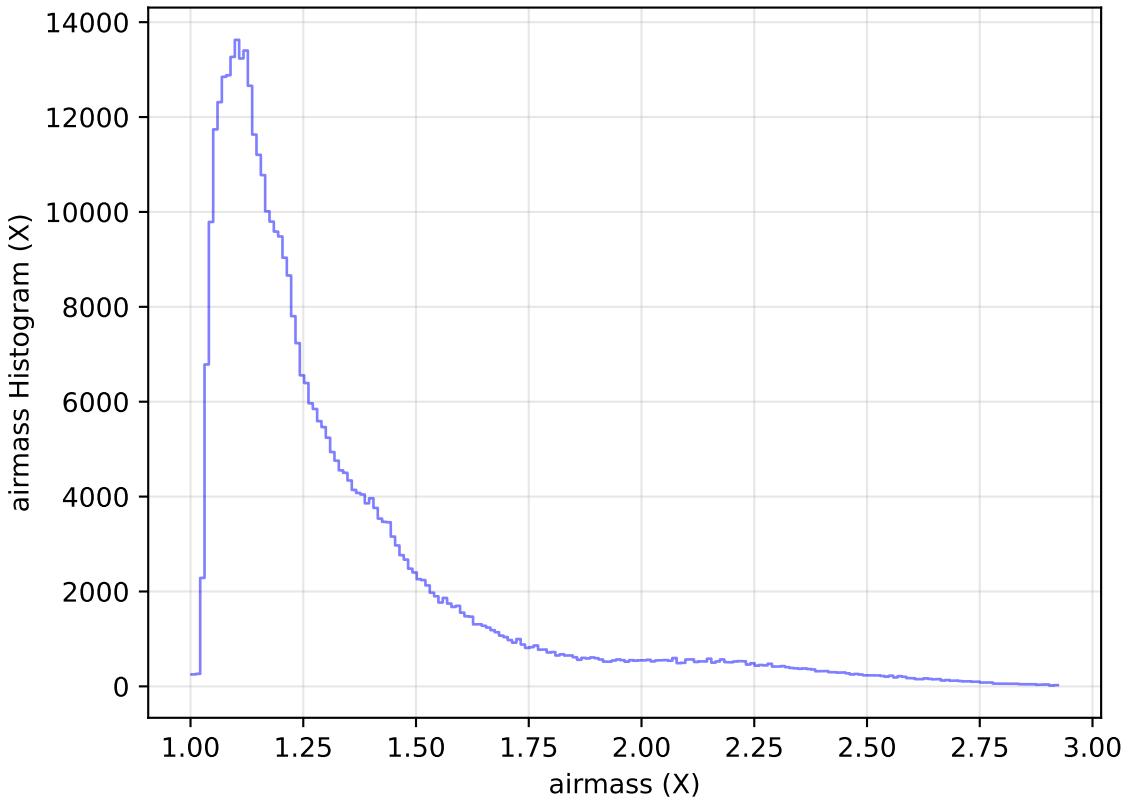
too_elab_r32_d3_ugrizy_v3.4_10yrs WFD z band: airmass Histogram
