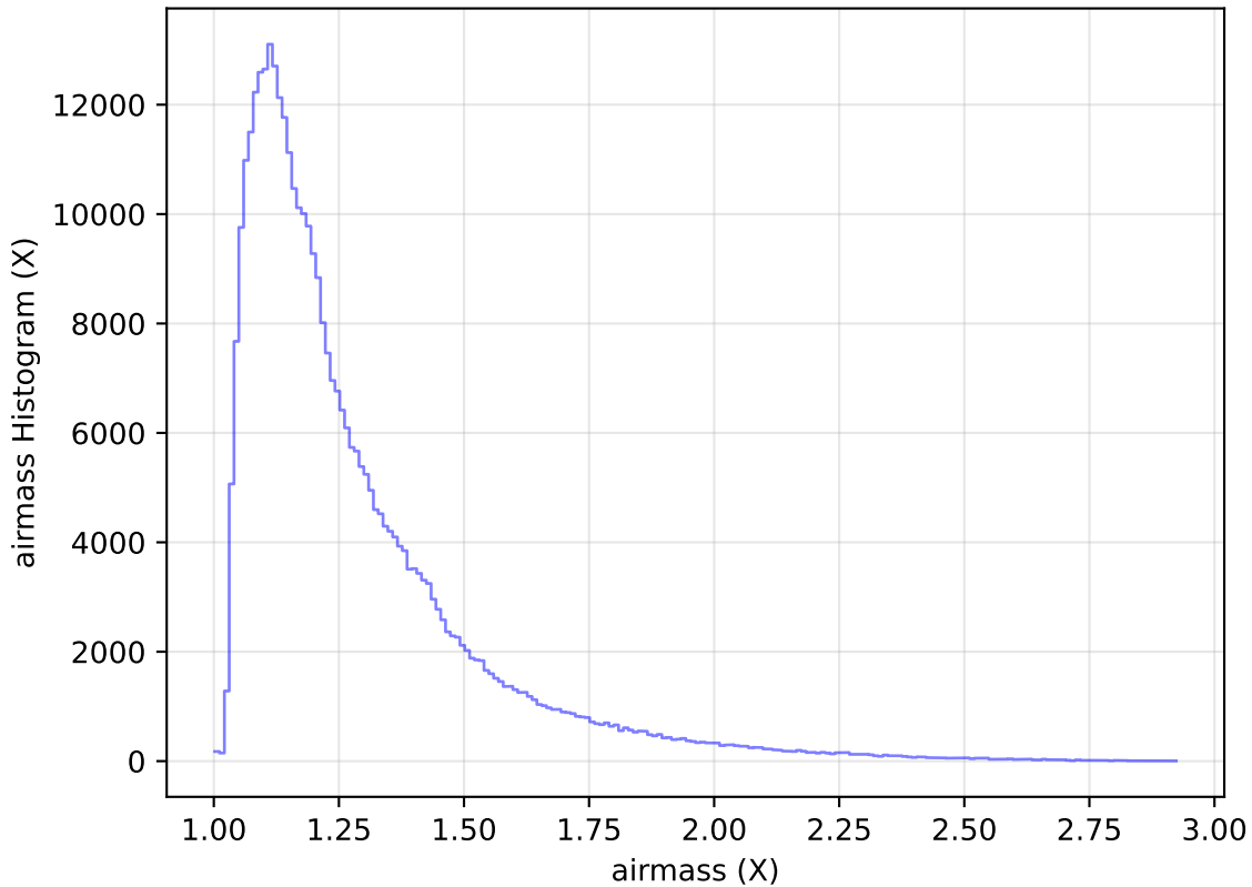
too_elab_r32_d3_ugrizy_v3.4_10yrs WFD y band: airmass Histogram
