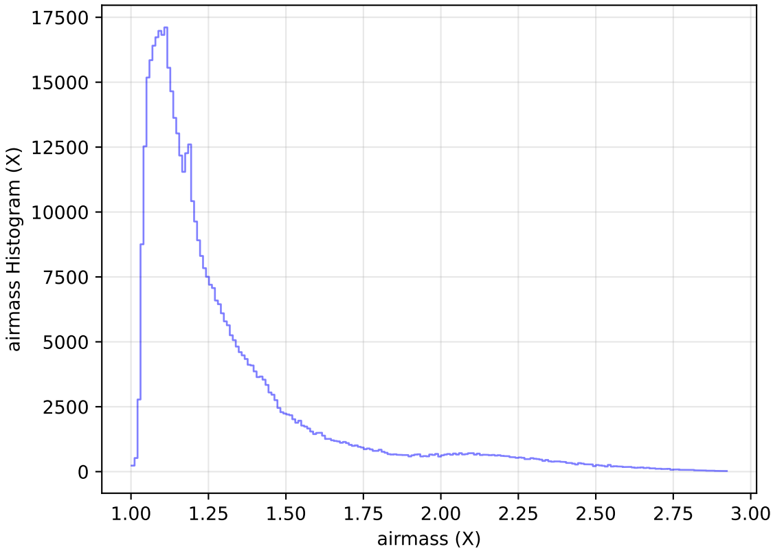
too_elab_r32_d3_ugrizy_v3.4_10yrs WFD i band: airmass Histogram
