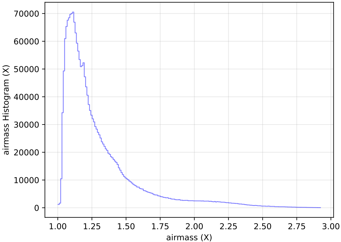
too_elab_r32_d3_ugrizy_v3.4_10yrs WFD all bands: airmass Histogram
