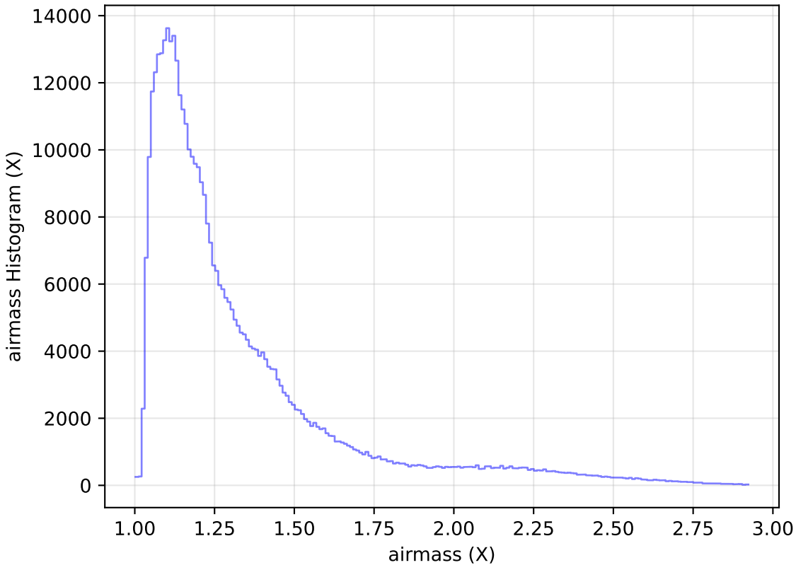
too_elab_r32_d3_ugrizy_v3.4_10yrs All sky z band: airmass Histogram
