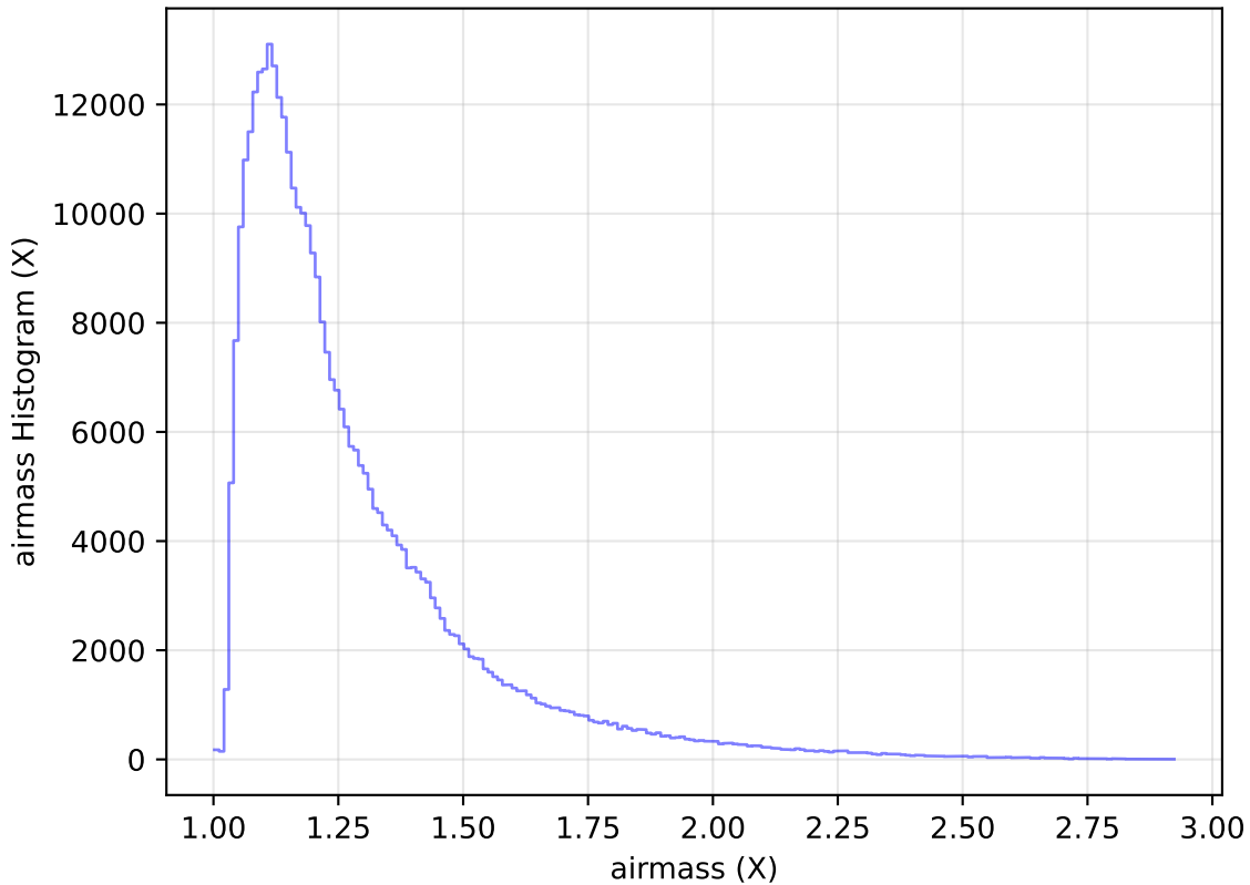
too_elab_r32_d3_ugrizy_v3.4_10yrs All sky y band: airmass Histogram
