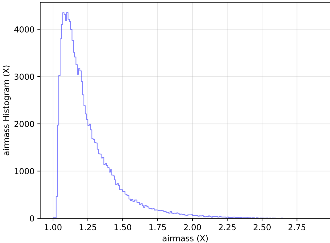
too_elab_r32_d3_ugrizy_v3.4_10yrs All sky u band: airmass Histogram
