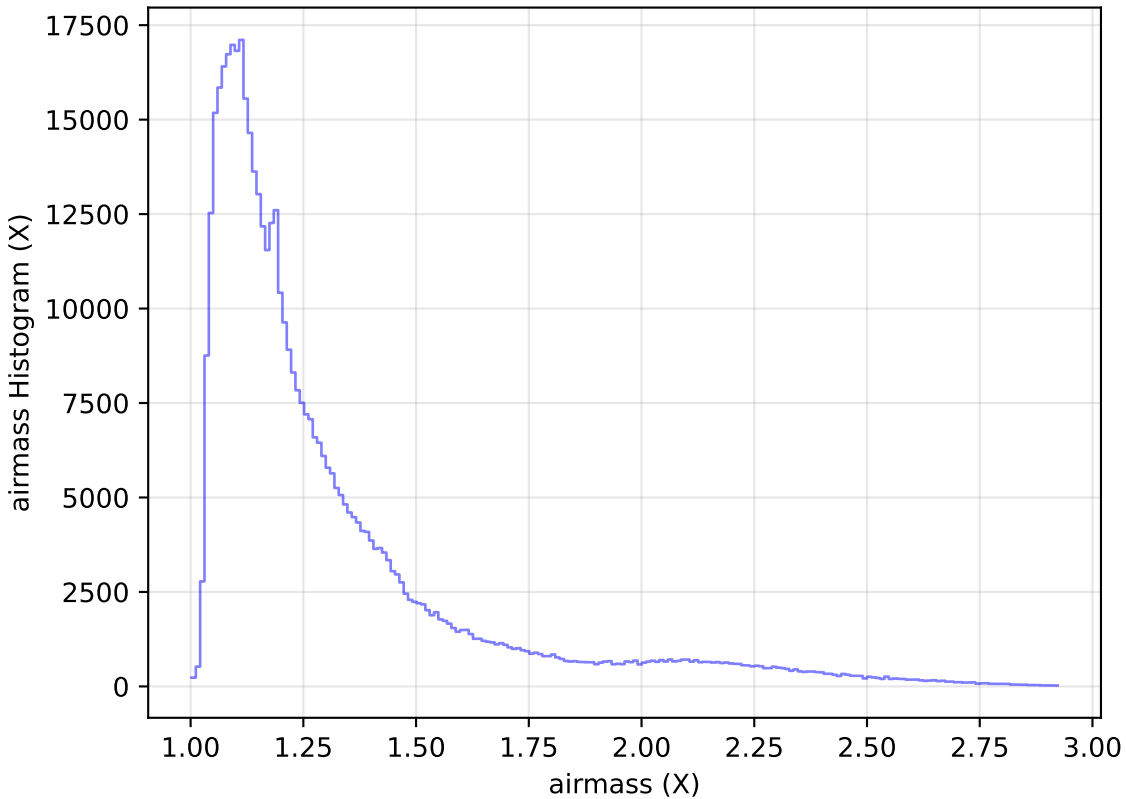
too_elab_r32_d3_ugrizy_v3.4_10yrs All sky i band: airmass Histogram
