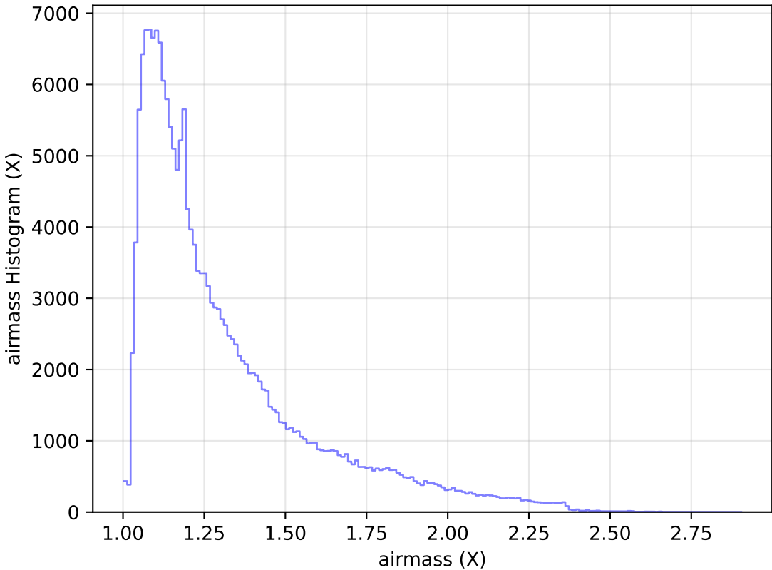
too_elab_r32_d3_ugrizy_v3.4_10yrs All sky g band: airmass Histogram
