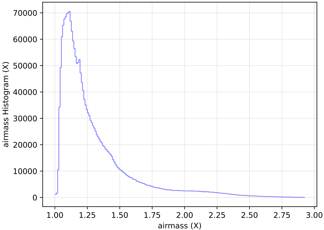
too_elab_r32_d3_ugrizy_v3.4_10yrs All sky all bands: airmass Histogram
