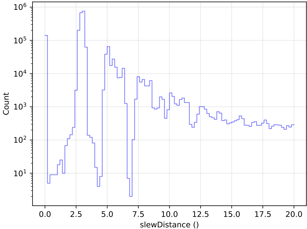
too_elab_r32_d3_ugrizy_v3.4_10yrs All visits: Zoom Slew Distance Histogram
