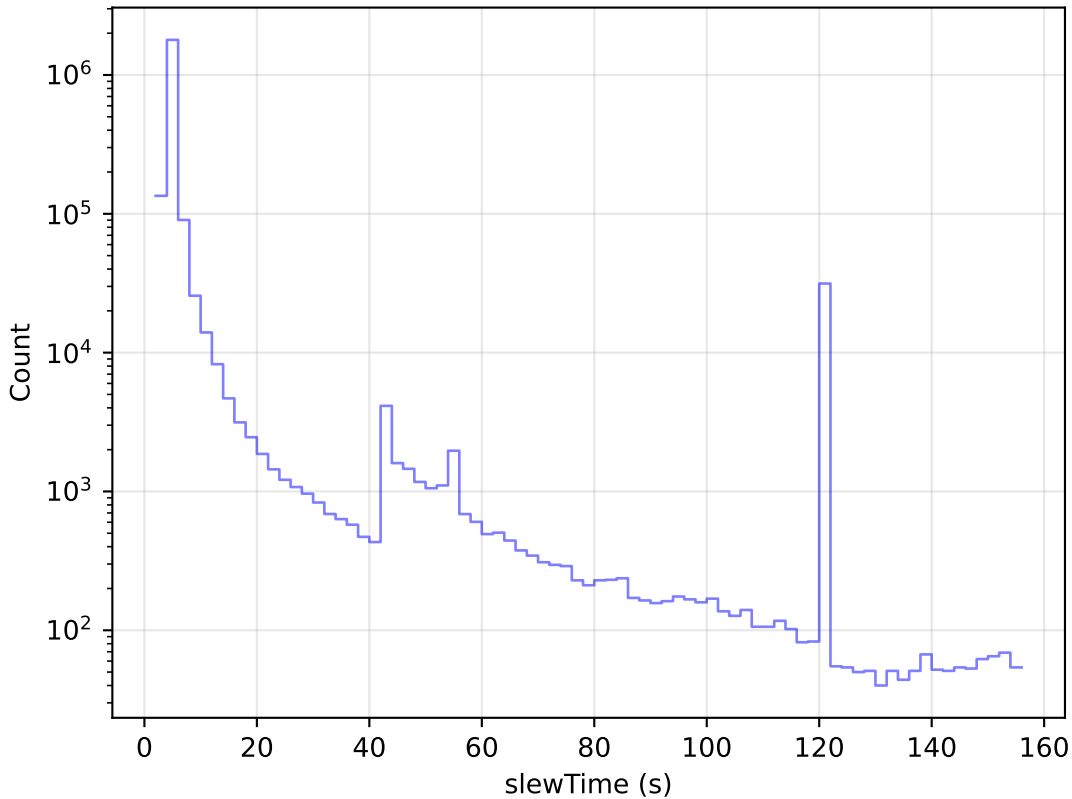
too_elab_r32_d3_ugrizy_v3.4_10yrs All visits: Slew Time Histogram
