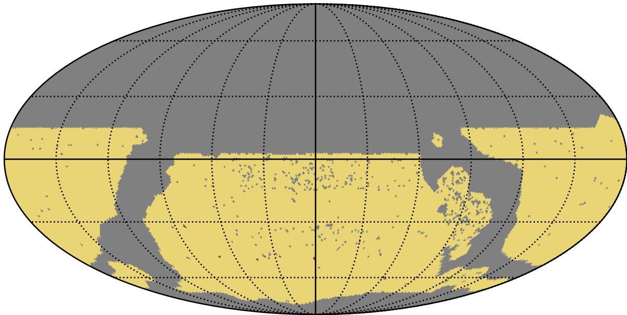
too_elab_r32_d3_ugrizy_v3.4_10yrs WFD: RapidRevisits
