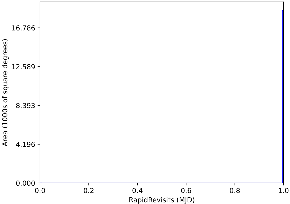
too_elab_r32_d3_ugrizy_v3.4_10yrs WFD: RapidRevisits
