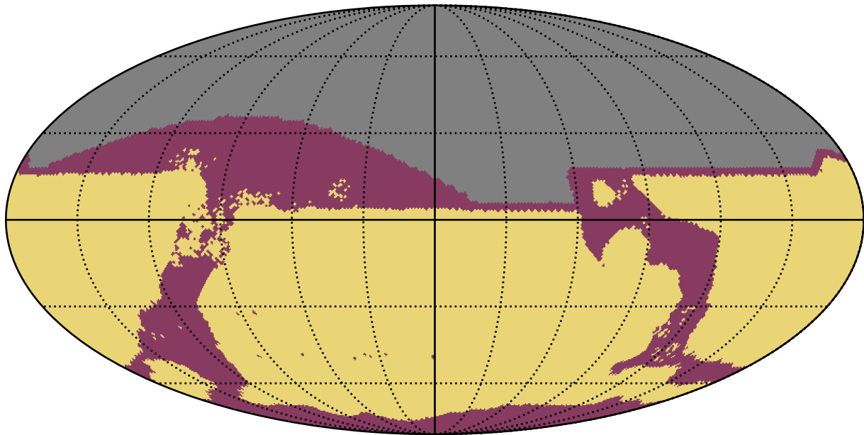
too_elab_r32_d3_ugrizy_v3.4_10yrs All sky: RapidRevisits
