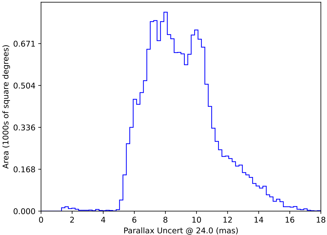
too_elab_r32_d3_ugrizy_v3.4_10yrs WFD: Parallax Uncert @ 24.0
