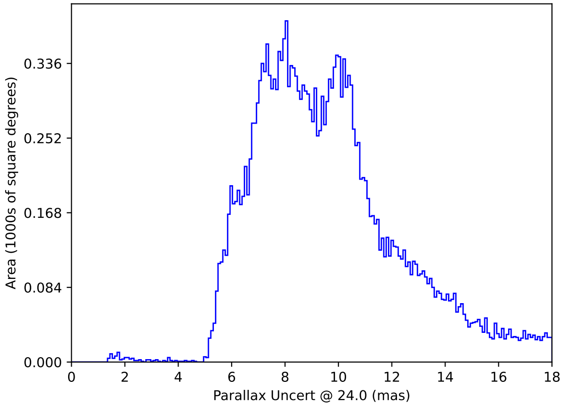
too_elab_r32_d3_ugrizy_v3.4_10yrs All sky: Parallax Uncert @ 24.0
