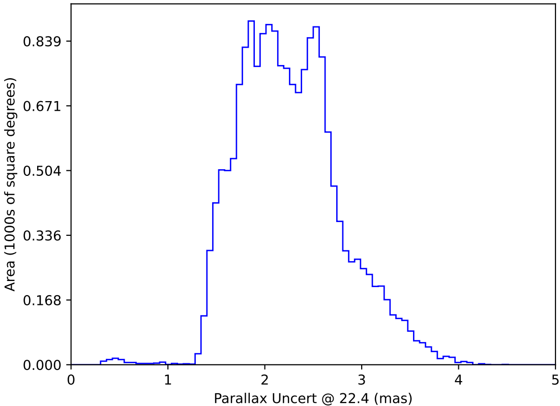
too_elab_r32_d3_ugrizy_v3.4_10yrs WFD: Parallax Uncert @ 22.4
