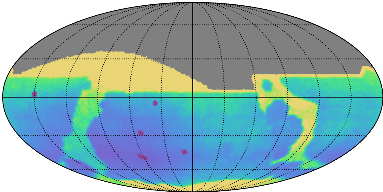
too_elab_r32_d3_ugrizy_v3.4_10yrs All sky: Parallax Uncert @ 22.4
