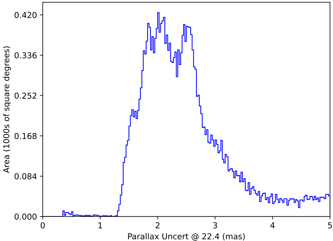
too_elab_r32_d3_uigrizy_v3.4_10yrs All sky: Parallax Uncert @ 22.4
