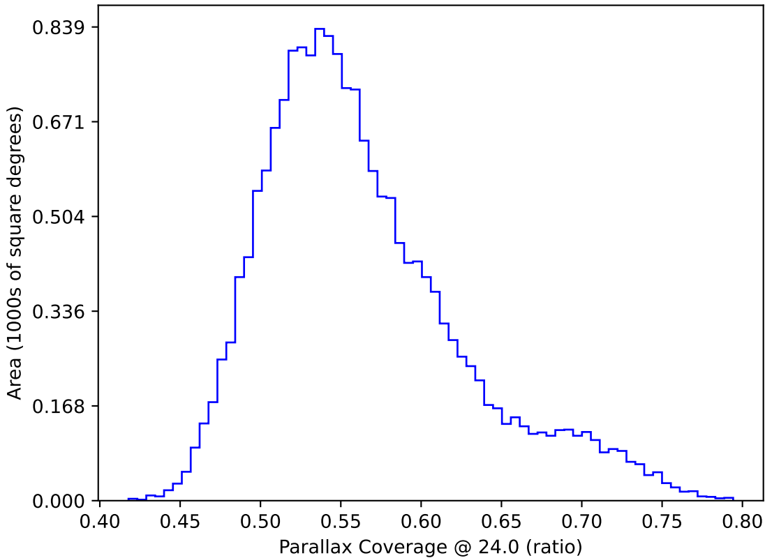
too_elab_r32_d3_ugrizy_v3.4_10yrs WFD: Parallax Coverage @ 24.0
