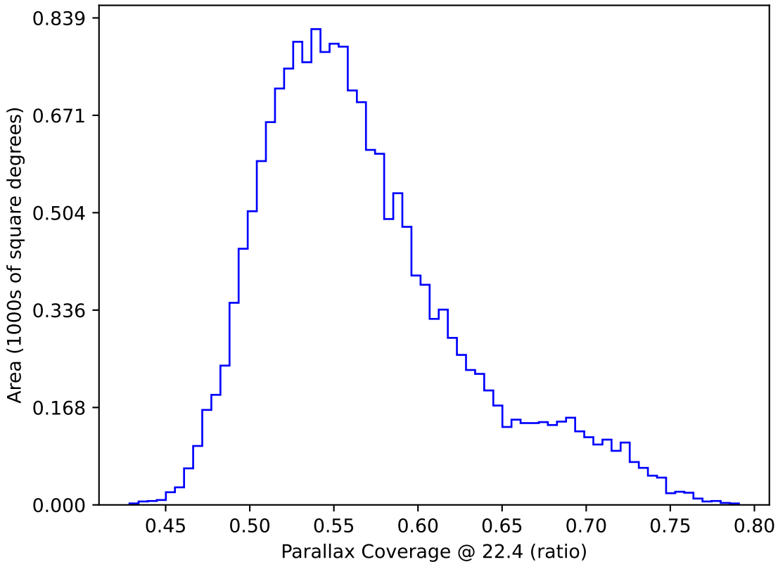
too_elab_r32_d3_ugrizy_v3.4_10yrs WFD: Parallax Coverage @ 22.4
