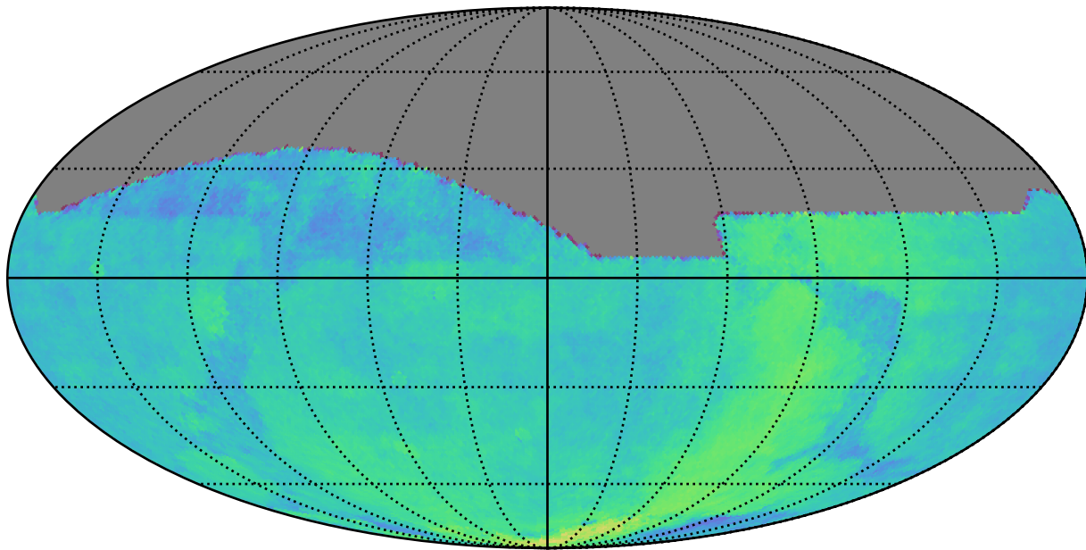
too_elab_r32_d3_ugrizy_v3.4_10yrs All sky: Parallax Coverage @ 22.4
