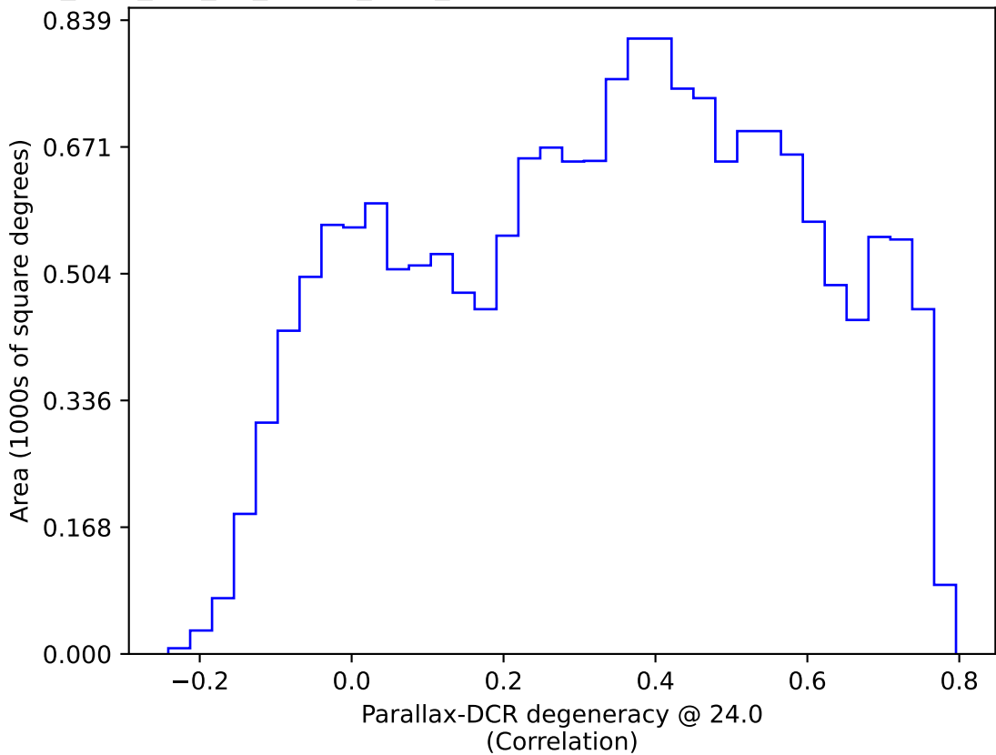
too_elab_r32_d3_ugrizy_v3.4_10yrs WFD: Parallax-DCR degeneracy @ 24.0
