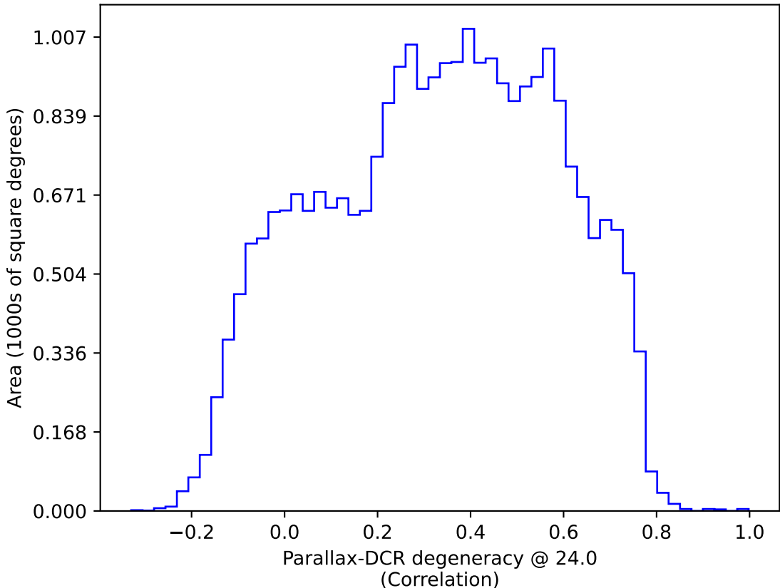
too_elab_r32_d3_ugrizy_v3.4_10yrs All sky: Parallax-DCR degeneracy @ 24.0
