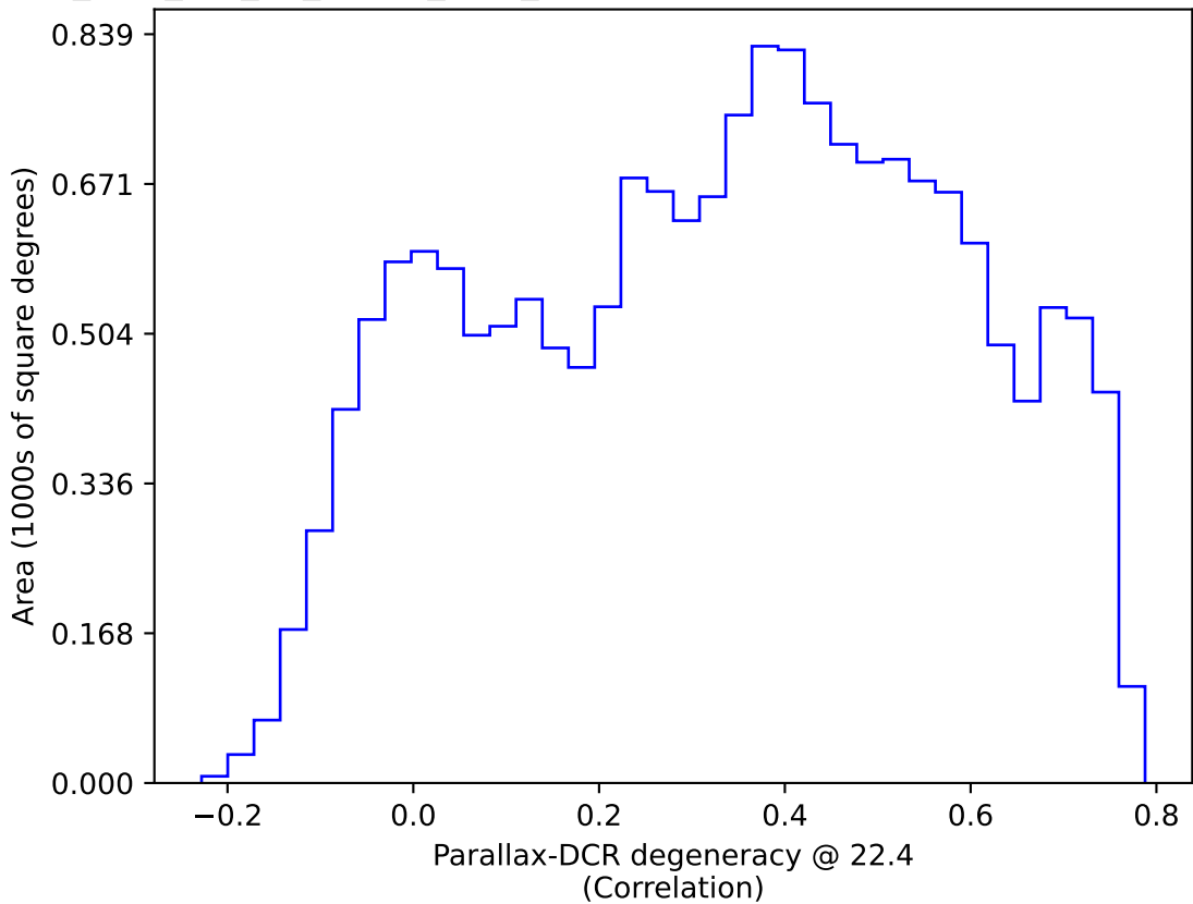
too_elab_r32_d3_ugrizy_v3.4_10yrs WFD: Parallax-DCR degeneracy @ 22.4
