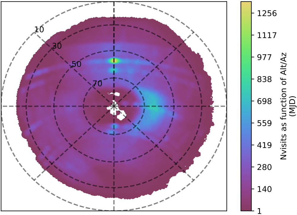
too_elab_r32_d3_ugrizy_v3.4_10yrs g band: Nvisits as function of Alt/Az
