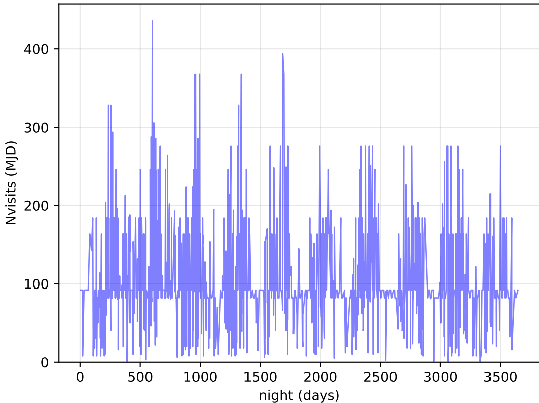
too_elab_r32_d3_ugrizy_v3.4_10yrs DDF: Nvisits
