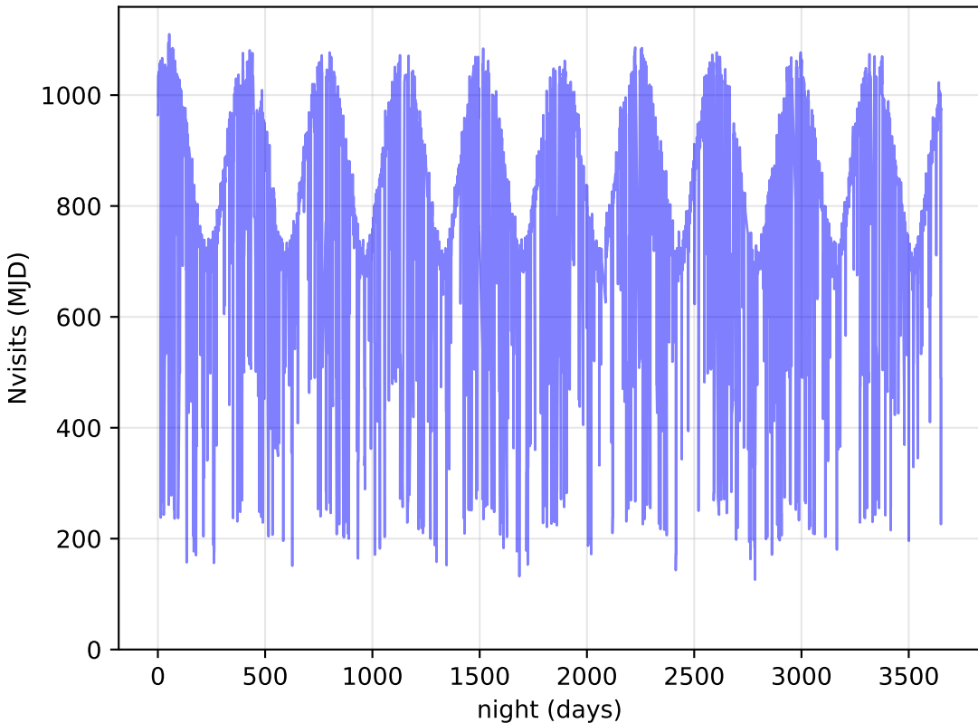
too_elab_r32_d3_ugrizy_v3.4_10yrs All visits: Nvisits
