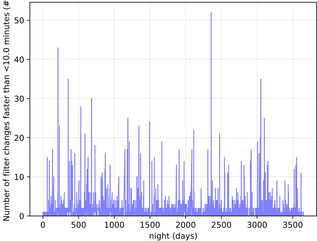
too_elab_r32_d3_ugrizy_v3.4_10yrs Per Night: Number of filter changes faster than <10.0 minutes
