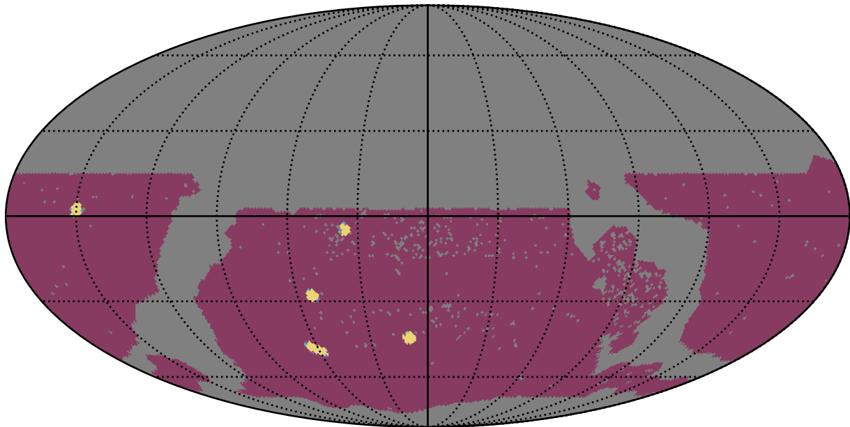
too_elab_r32_d3_ugrizy_v3.4_10yrs WFD: NumberOfQuickRevisits
