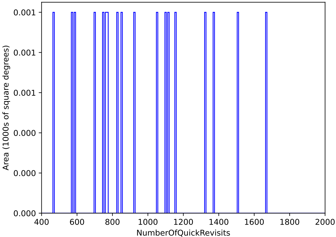
too_elab_r32_d3_ugrizy_v3.4_10yrs WFD: NumberOfQuickRevisits
