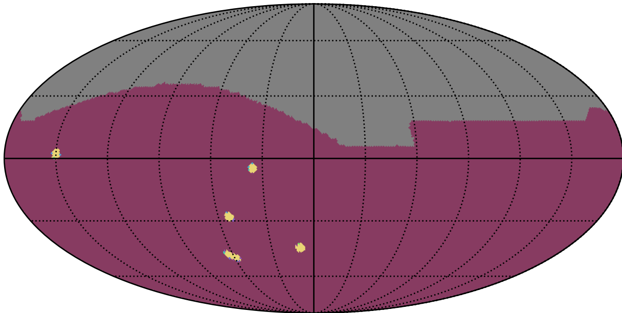
too_elab_r32_d3_ugrizy_v3.4_10yrs All sky: NumberOfQuickRevisits
