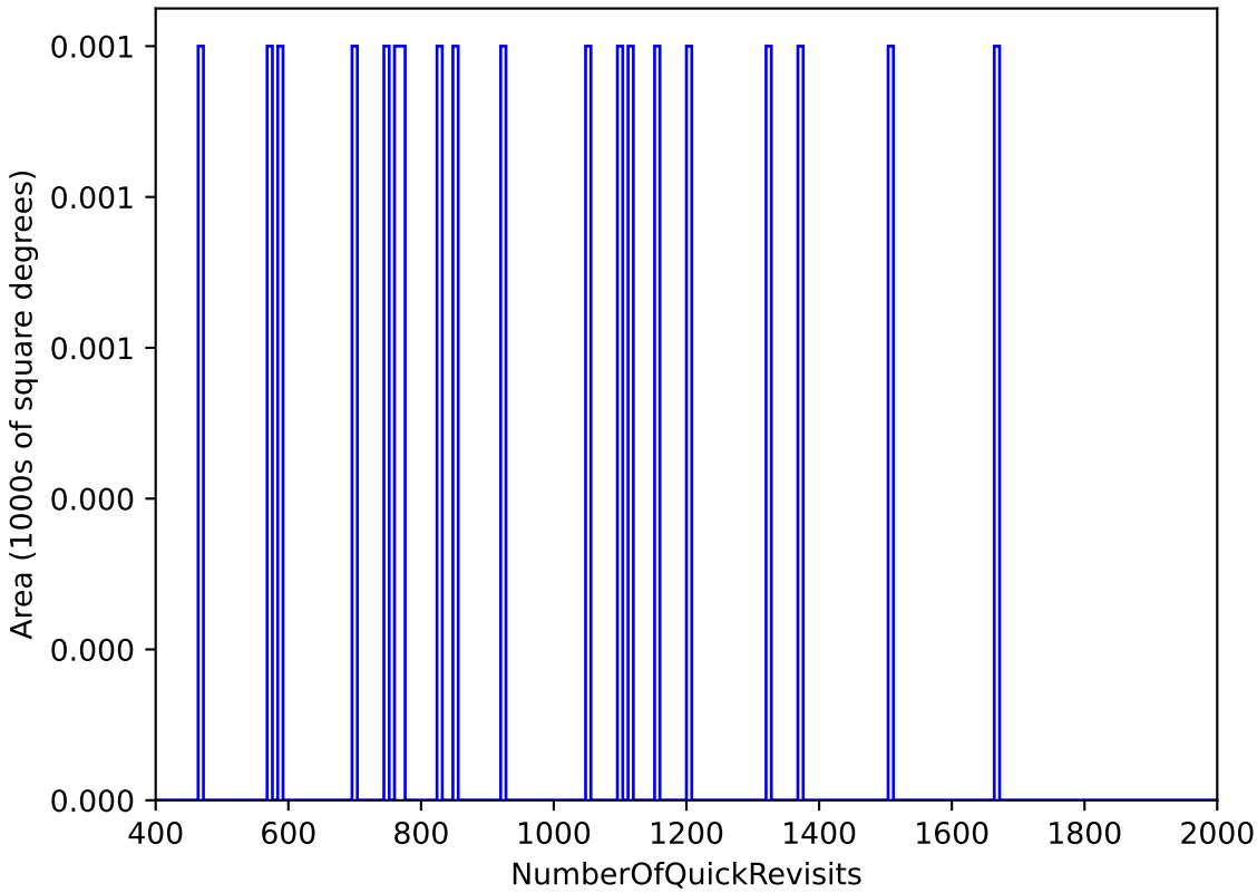
too_elab_r32_d3_ugrizy_v3.4_10yrs All sky: NumberOfQuickRevisits
