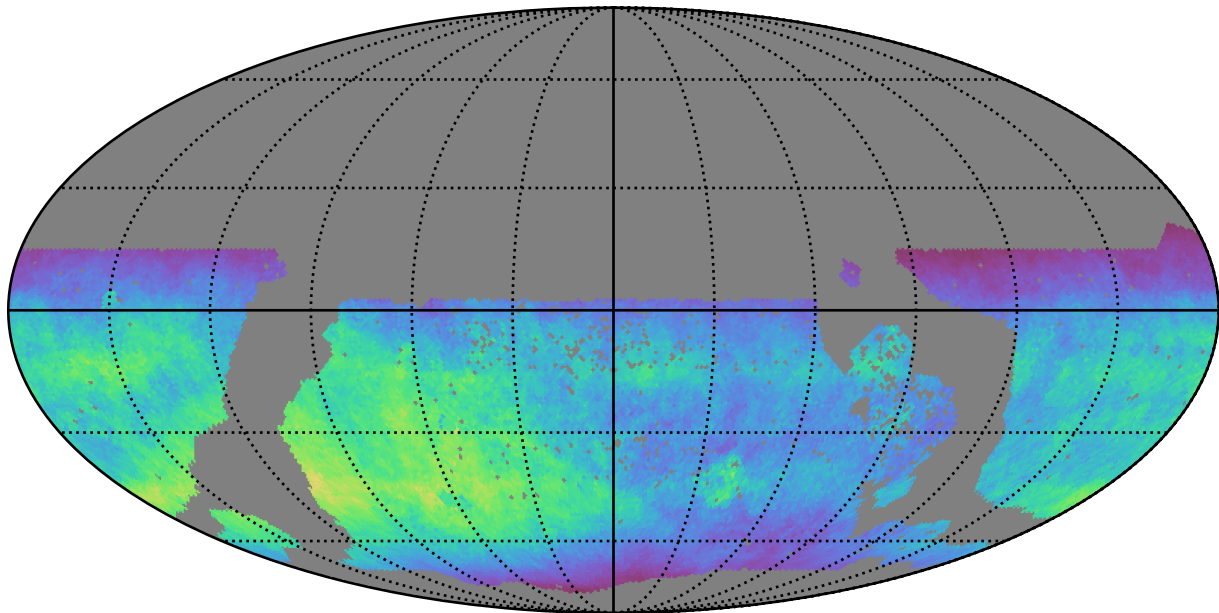
too_elab_r32_d3_ugrizy_v3.4_10yrs WFD z band: Normalized Teff
