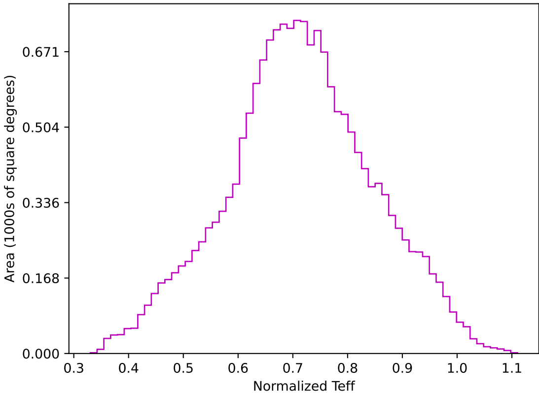
too_elab_r32_d3_ugrizy_v3.4_10yrs WFD z band: Normalized Teff
