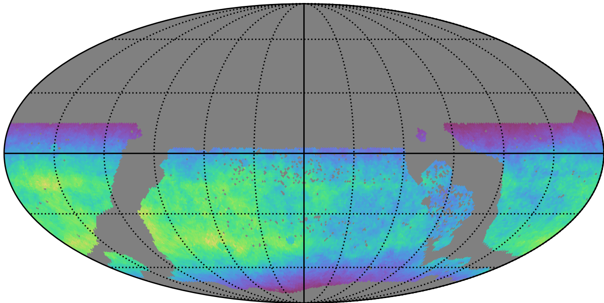
too_elab_r32_d3_ugrizy_v3.4_10yrs WFD y band: Normalized Teff
