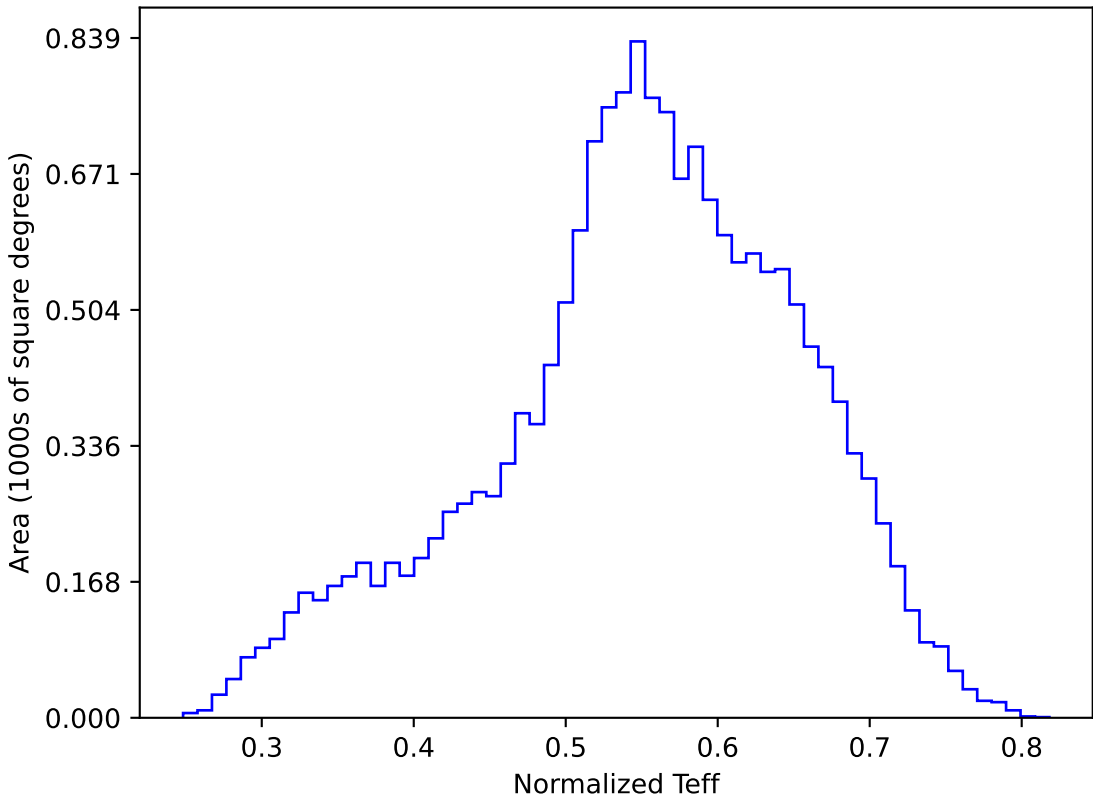
too_elab_r32_d3_ugrizy_v3.4_10yrs WFD y band: Normalized Teff
